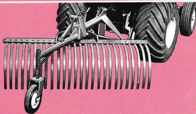
Material is discharged to either side after simple angle adjustment. Three point hitch.
